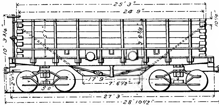
Fig. 67. Side Elevation.
